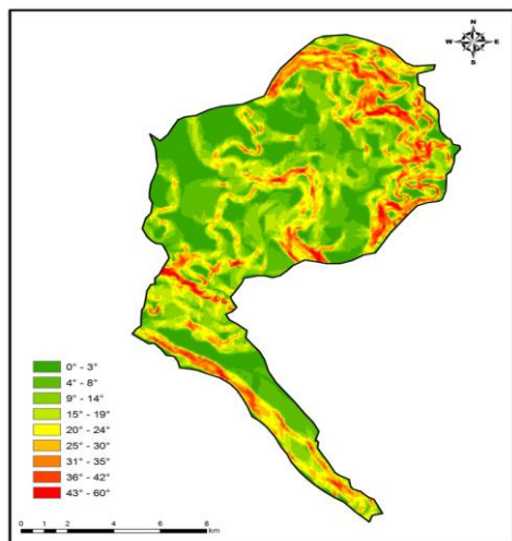
Sl. 9. Reljefna struktura Sutorine izražena nagibima Fig. 9. Relief structure of Sutorina expressed by terrain slopes
