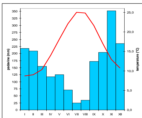
Sl. 11. Klima dijagram padavina (plavi stupci) i temperatura (crveni linijski grafikon) Fig 11. Climate diagram of percipitation (blue bars) and temperature (red line)
