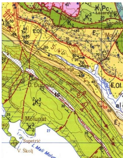
Sl. 6. Geološka građa u poriječju Sutorine Fig. 6. Geological structure in drainage basin of Sutorina
